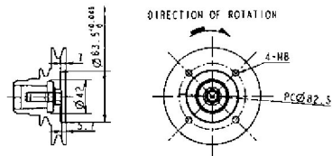
DETAIL OF PULLEY(A) (SCALE 1:3)
